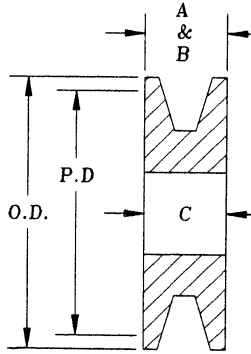
FIXED BORE TYPE
